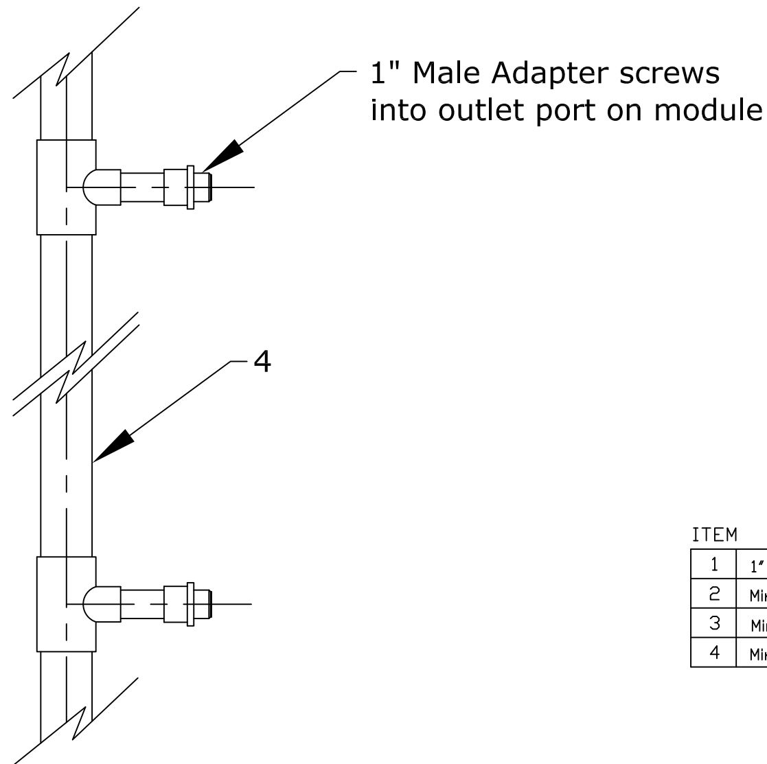
PARTIAL ASSEMBLY
